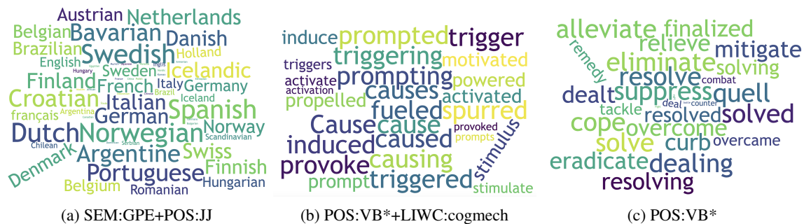
Figure 5: Examples of unaligned encoded concepts: (a) combination of geopolitical entities and their related adjectives, (b,c) different forms of verb with specific semantics
