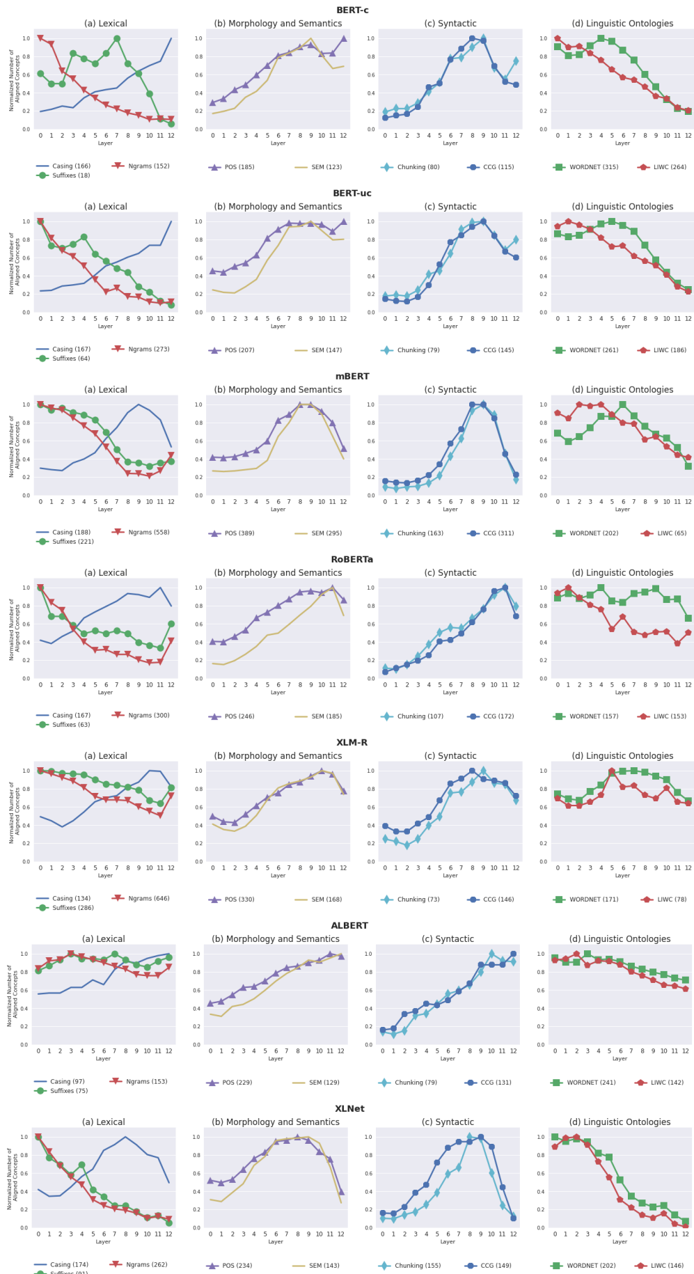
Figure 10: Layer-wise results.
