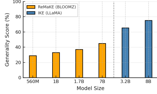
Figure 3: Generality scores for BLOOMZ and LLaMA models across increasing model sizes. ReMaKE (Wang et al., 2024c) (BLOOMZ) results are extracted for mzsRE generality, averaged across 10 languages. IKE (Nie et al., 2025) (LLaMA) results are extracted for mzsRE generality under zero-shot settings, averaged across 53 languages. Results show that generality consistently improves with model scale for both models.
