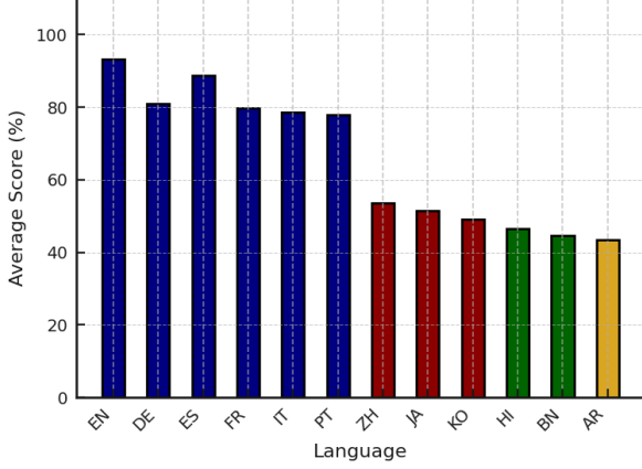
Figure 2: The figure shows average Reliability and Generality for MEMLA (Xie et al., 2024) across twelve languages, illustrating a typical directionality pattern: edits in high-resource or related languages transfer better than those in low-resource or distant ones.
