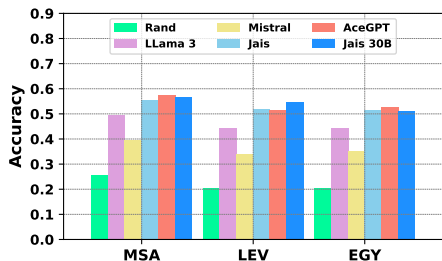
Figure 15: Average scores on ArabicMMLU
