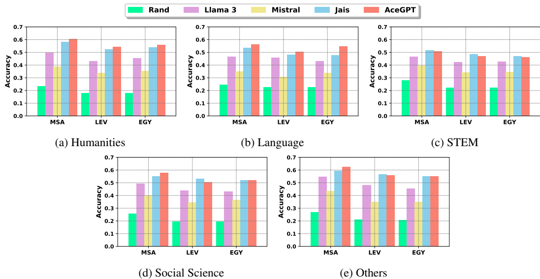
Figure 14: ArabicMMLU categories. Arabic alphabets prompt.
